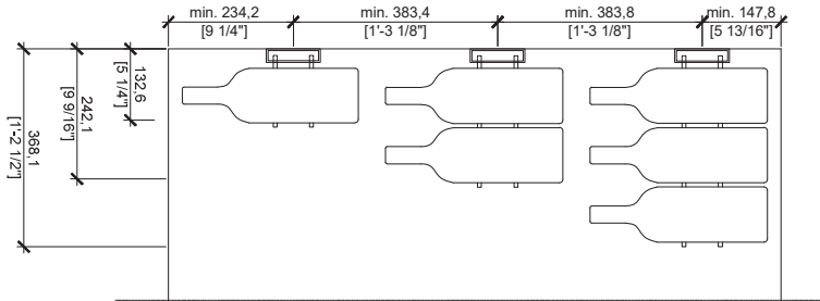
MAGNUM BOTTLE SPACING (M1, M2, M3)
