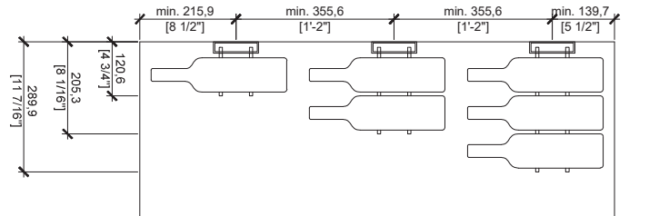
STANDARD BOTTLE SPACING (S1, S2, S3)
