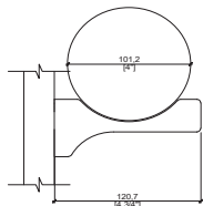
Magnum- 1 Bottle (M1)
