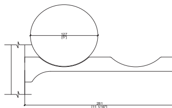
Double Magnum- 2 Bottle (DM2)
