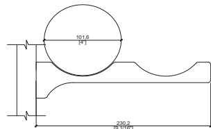
Magnum- 2 Bottle (M2)
