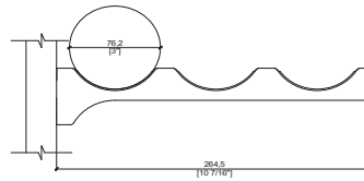
Standard - 3 Bottle (S3)
